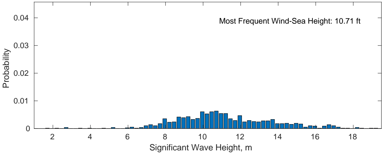
Wind-Sea: 11.81%
