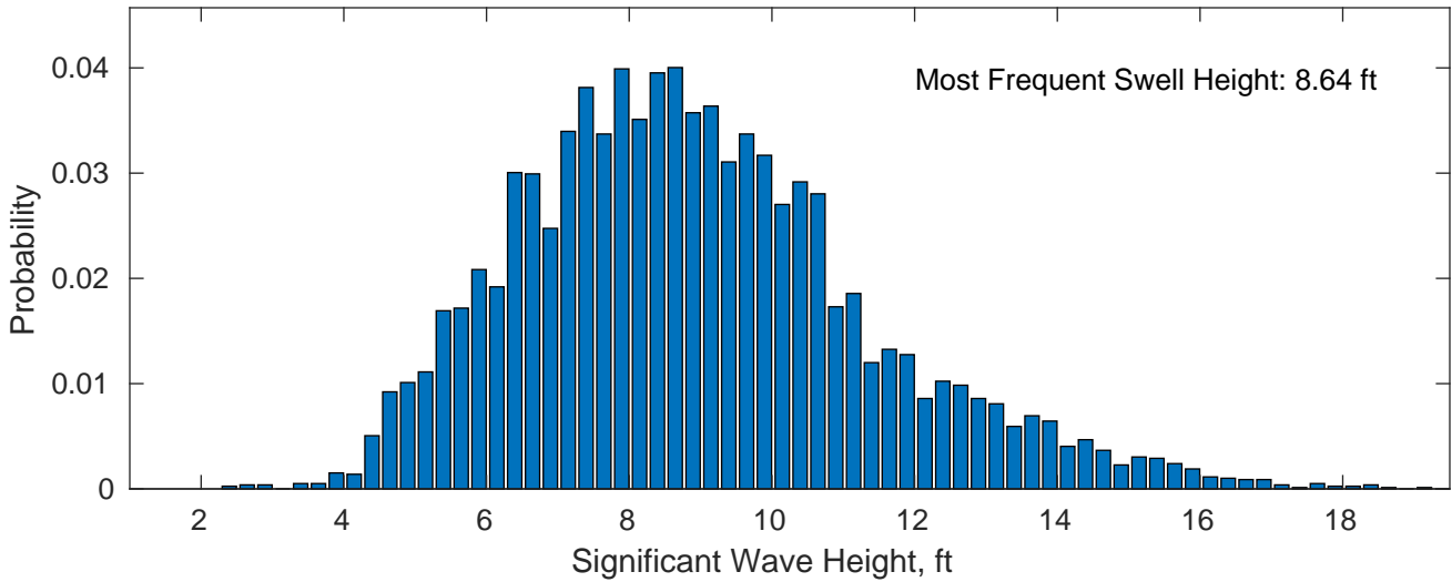
Swell: 88.19%
