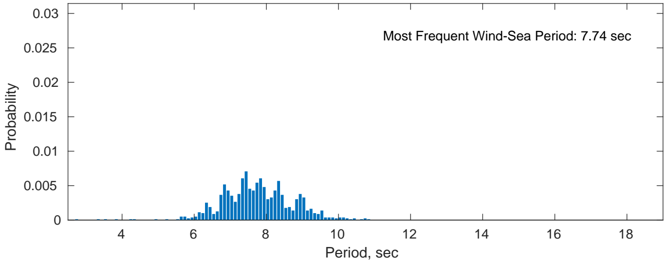
Wind-Sea: 11.81%
