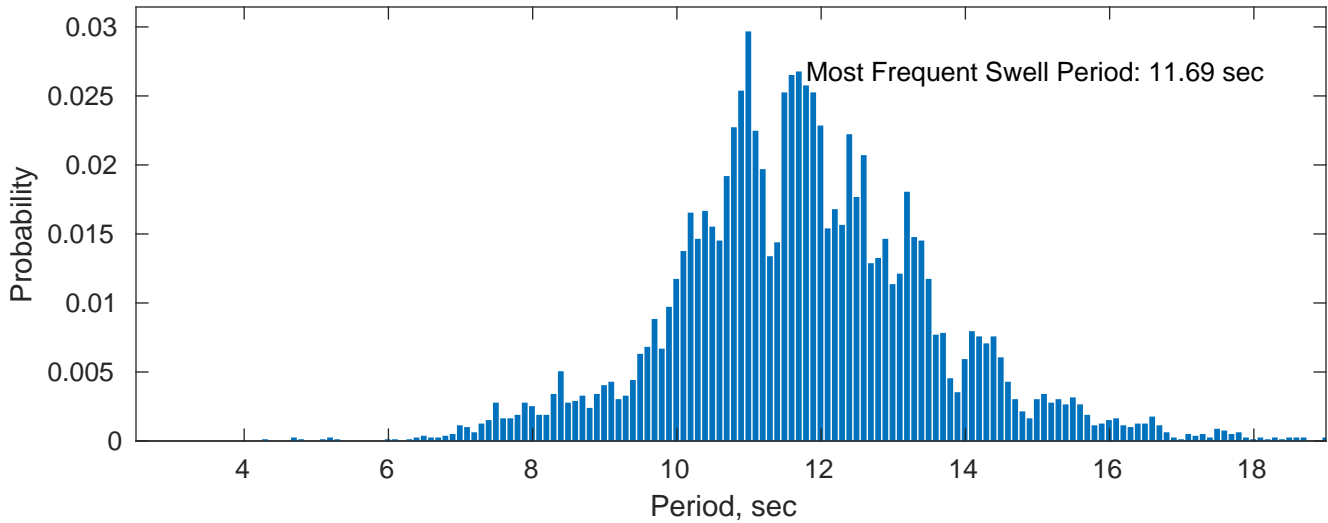
Swell: 88.19%
