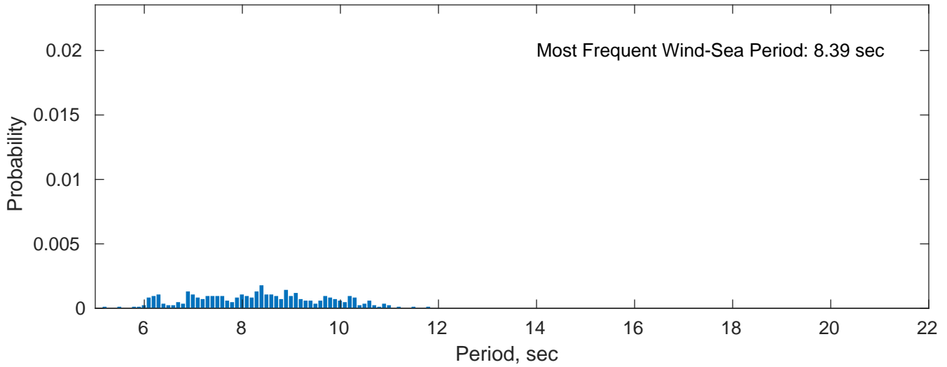
Wind-Sea: 3.89%
