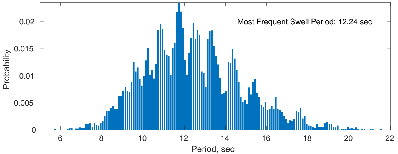
Swell: 96.11%
