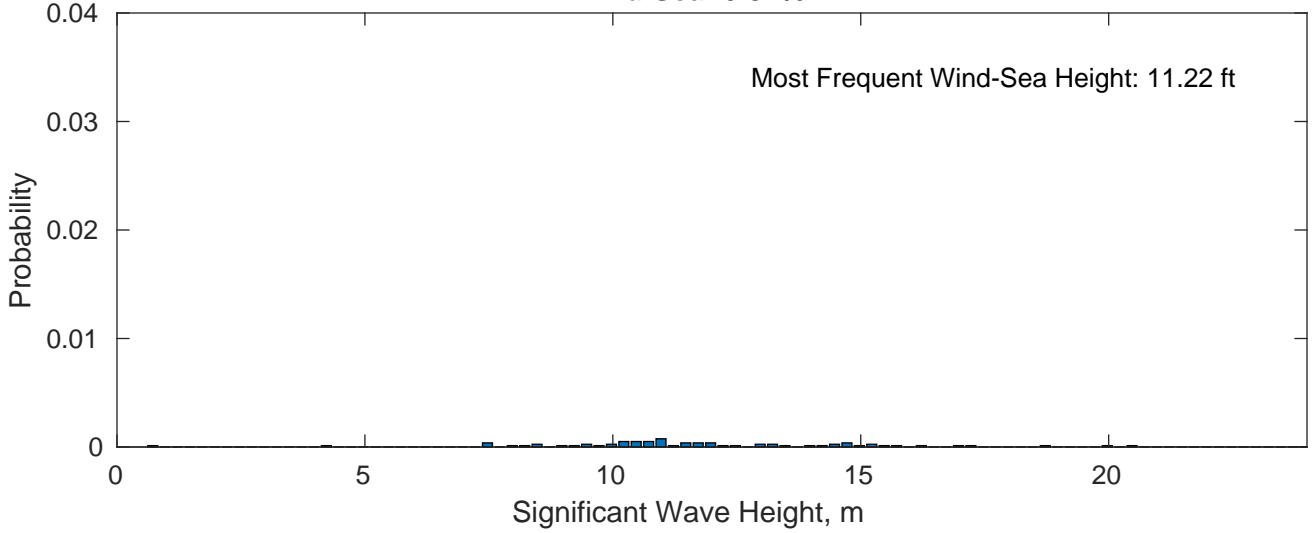
Wind-Sea: 0.87%
