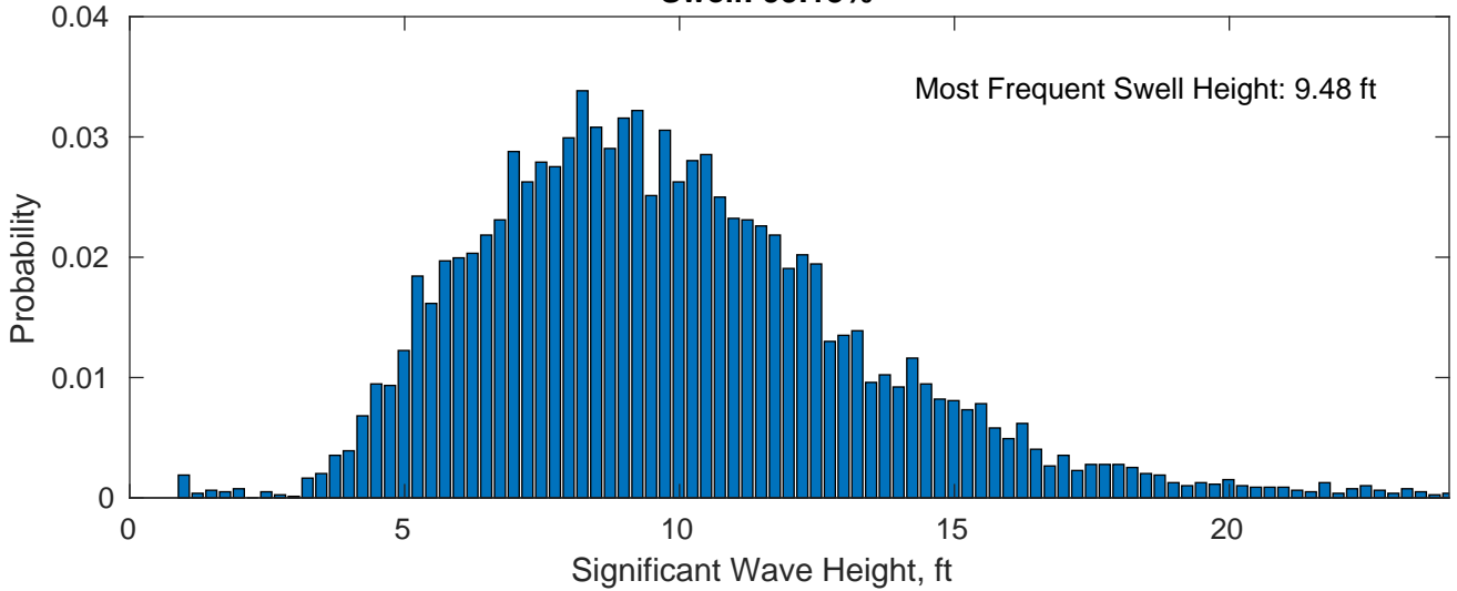
Swell: 99.13%
