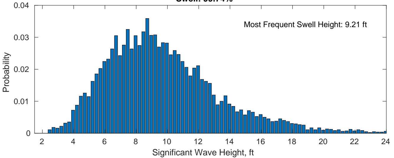
Swell: 99.74%
