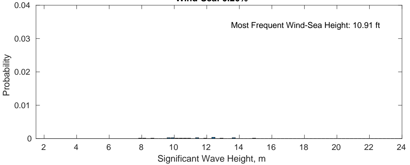
Wind-Sea: 0.26%
