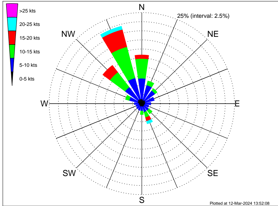
Even Keel Wind Project Climatological Wind Rose for January: 1979 - 2015
