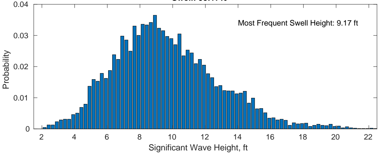
Swell: 99.17%
