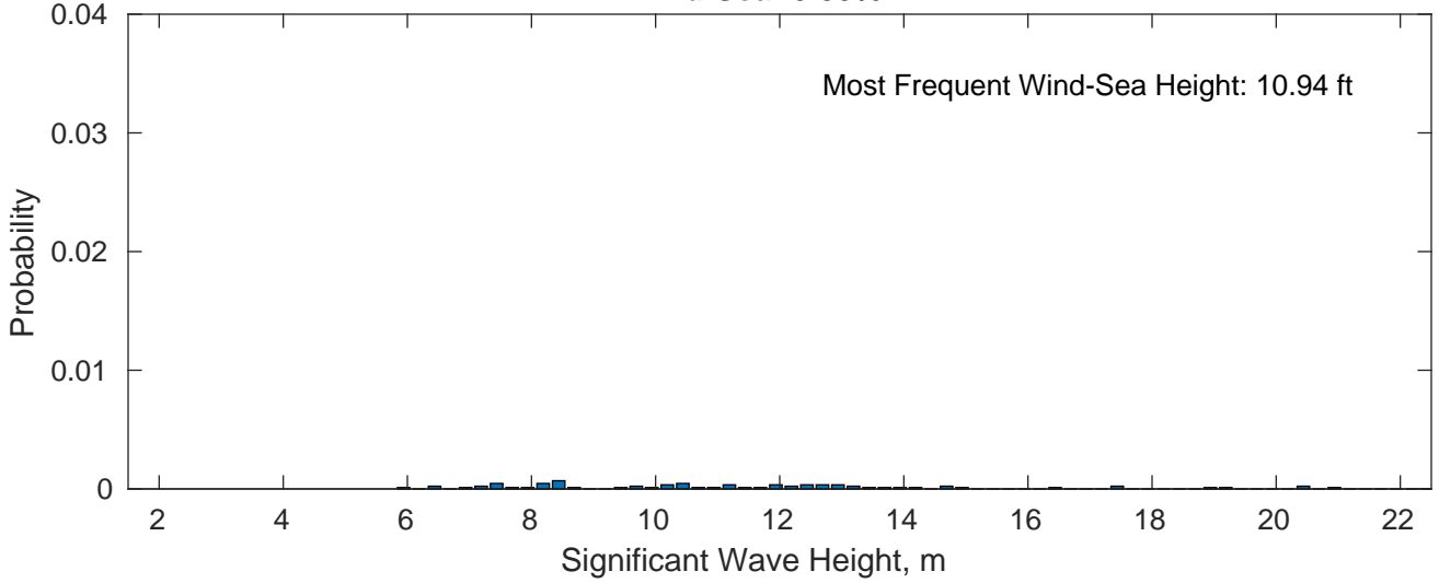
Wind-Sea: 0.83%
