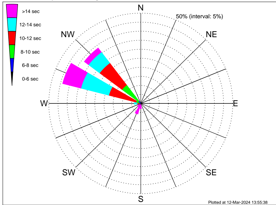
Even Keel Wind Project Climatological WavePeriod Rose for October: 1979 - 2015
