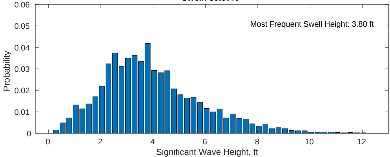
Swell: 59.97%
