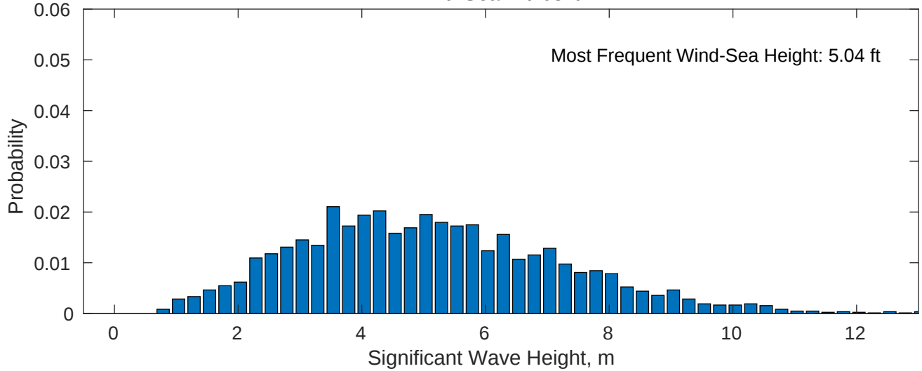
Wind-Sea: 40.03%
