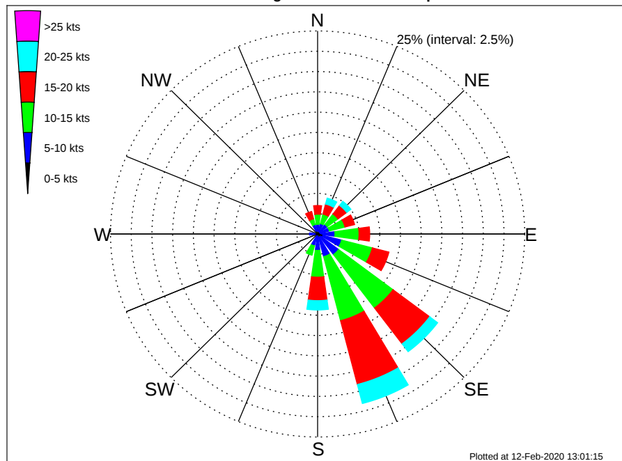
Flower Gardens NMS Climatological Wind Rose for April: 1979 - 2015
