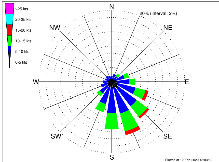
Flower Gardens NMS Climatological Wind Rose for August: 1979 - 2015
