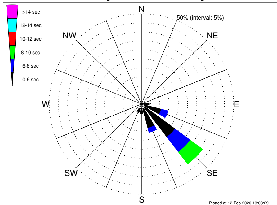
Flower Gardens NMS Climatological WavePeriod Rose for August: 1979 - 2015
