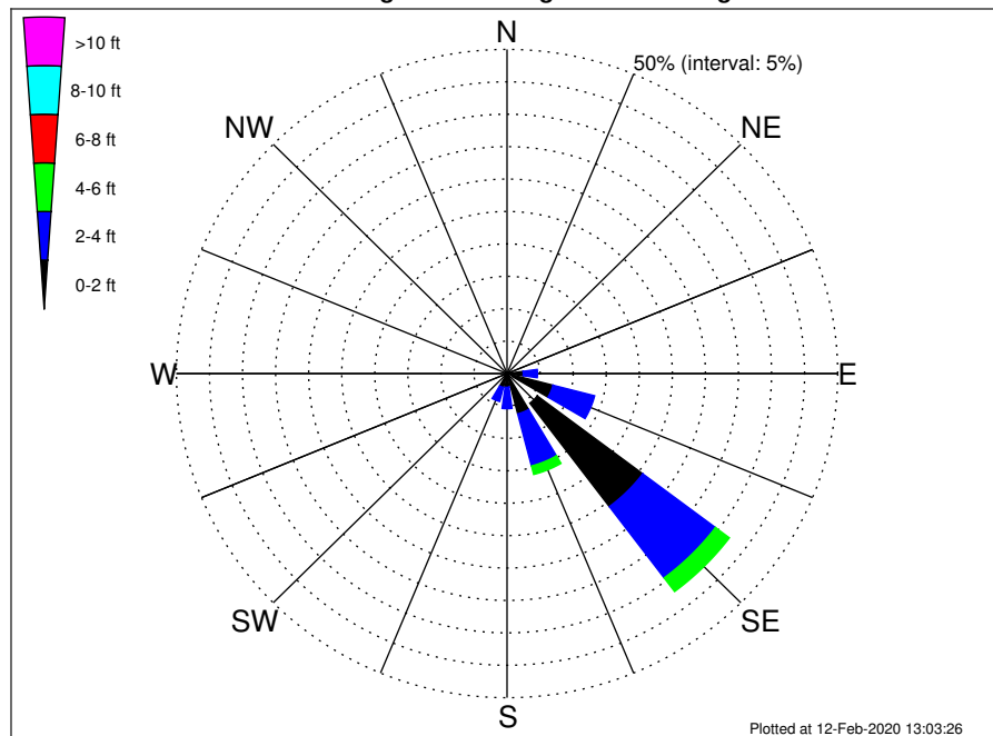
Flower Gardens NMS Climatological WaveHeight Rose for August: 1979 - 2015
