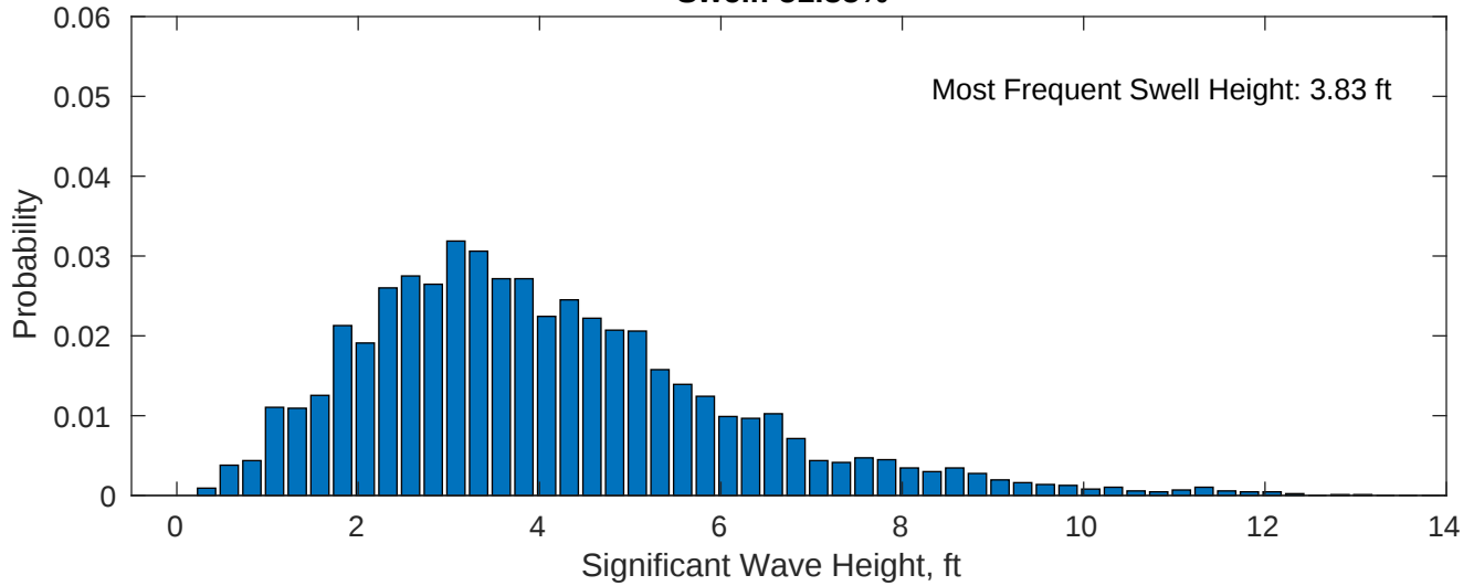
Swell: 51.35%
