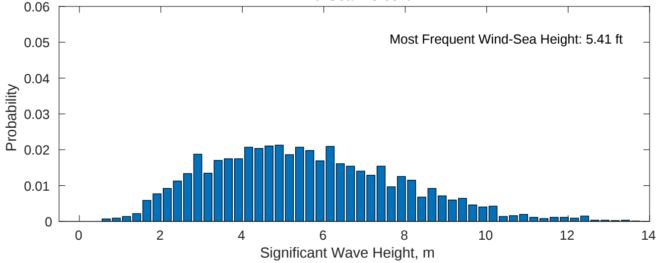
Wind-Sea: 48.65%
