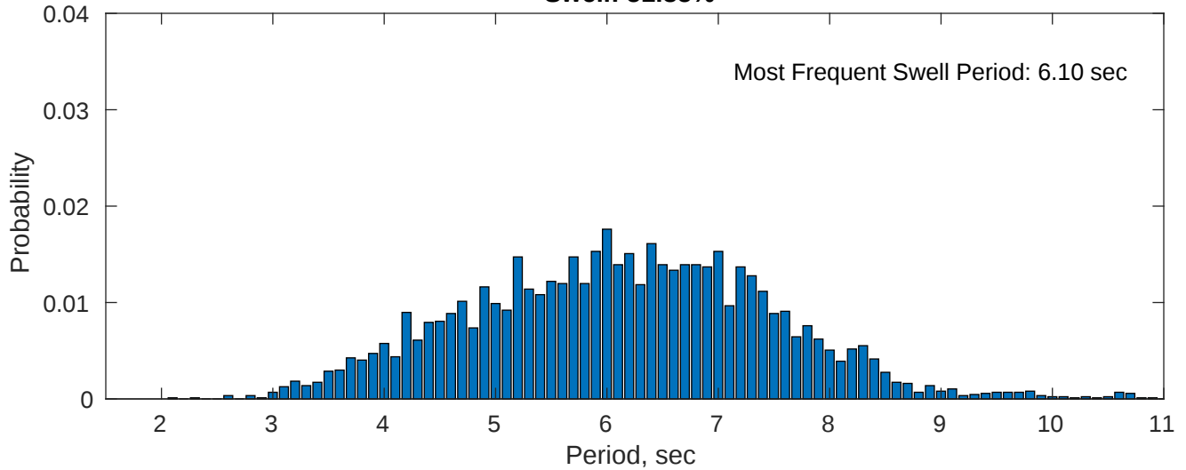
Swell: 51.35%
