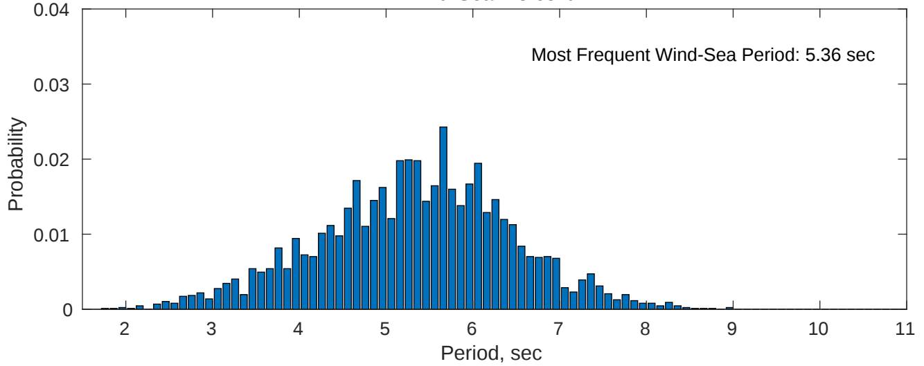
Wind-Sea: 48.65%
