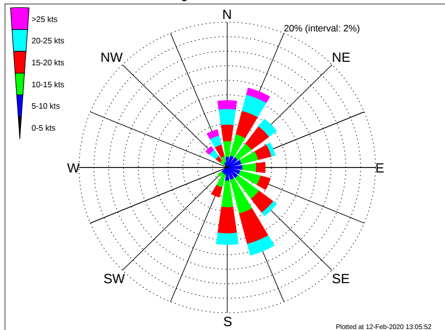
Flower Gardens NMS Climatological Wind Rose for December: 1979 - 2015
