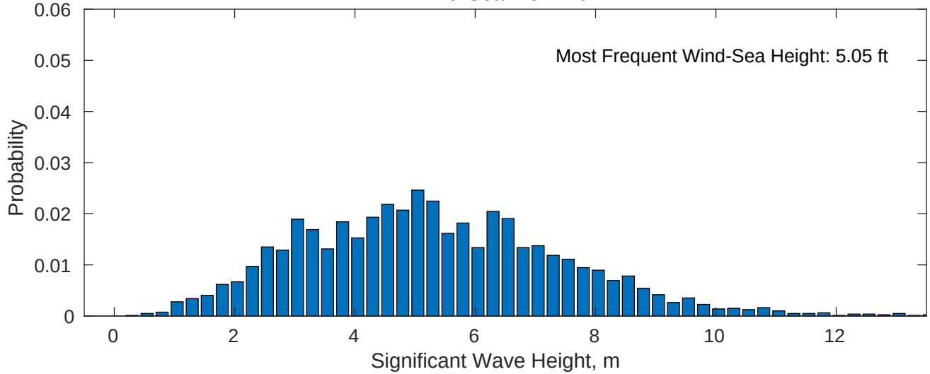
Wind-Sea: 45.21%
