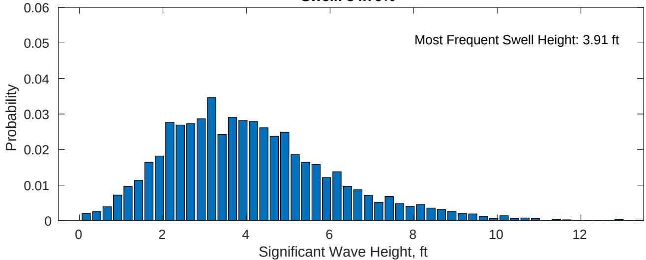
Swell: 54.79%
