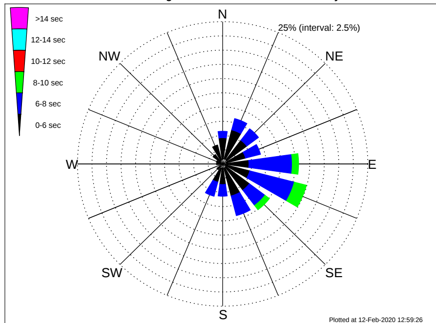
Flower Gardens NMS Climatological WavePeriod Rose for January: 1979 - 2015
