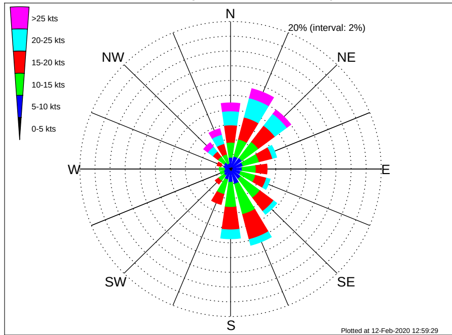
Flower Gardens NMS Climatological Wind Rose for January: 1979 - 2015
