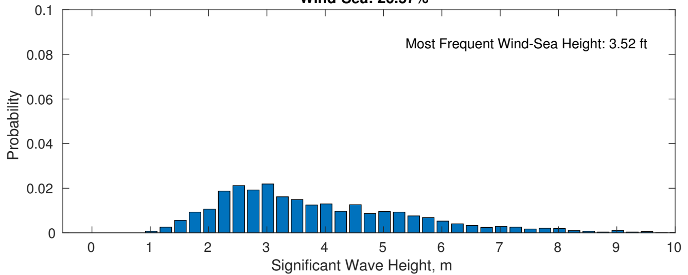
Wind-Sea: 26.57%
