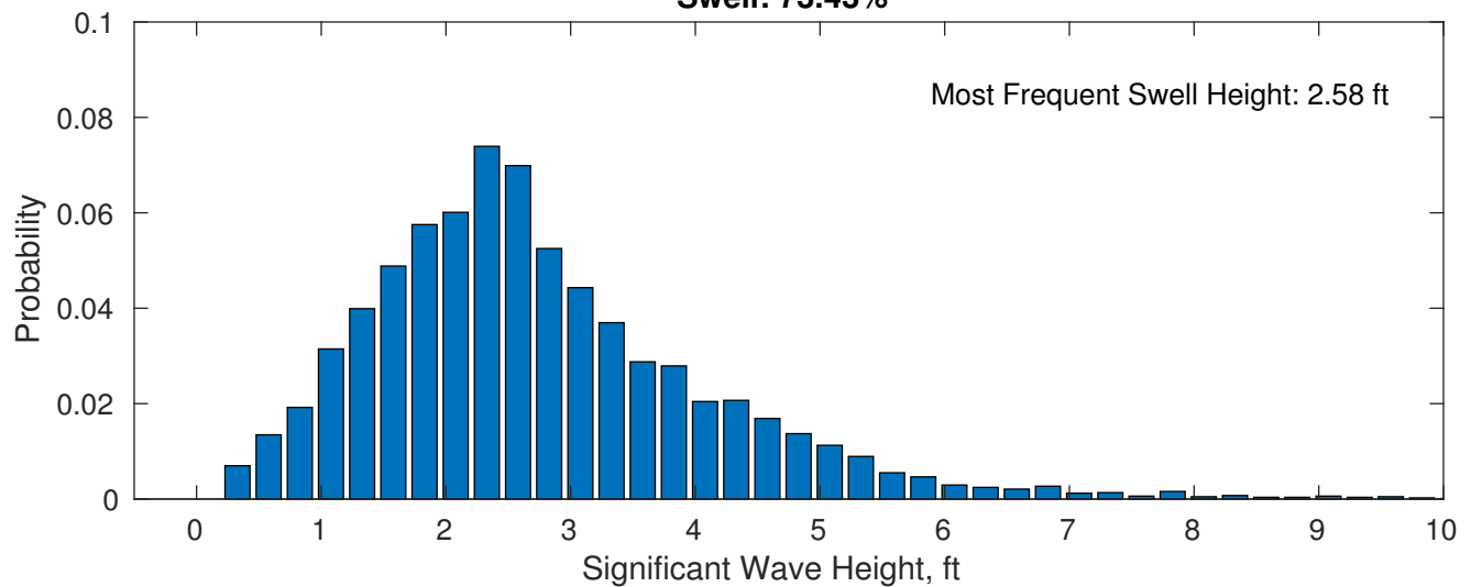
Swell: 73.43%
