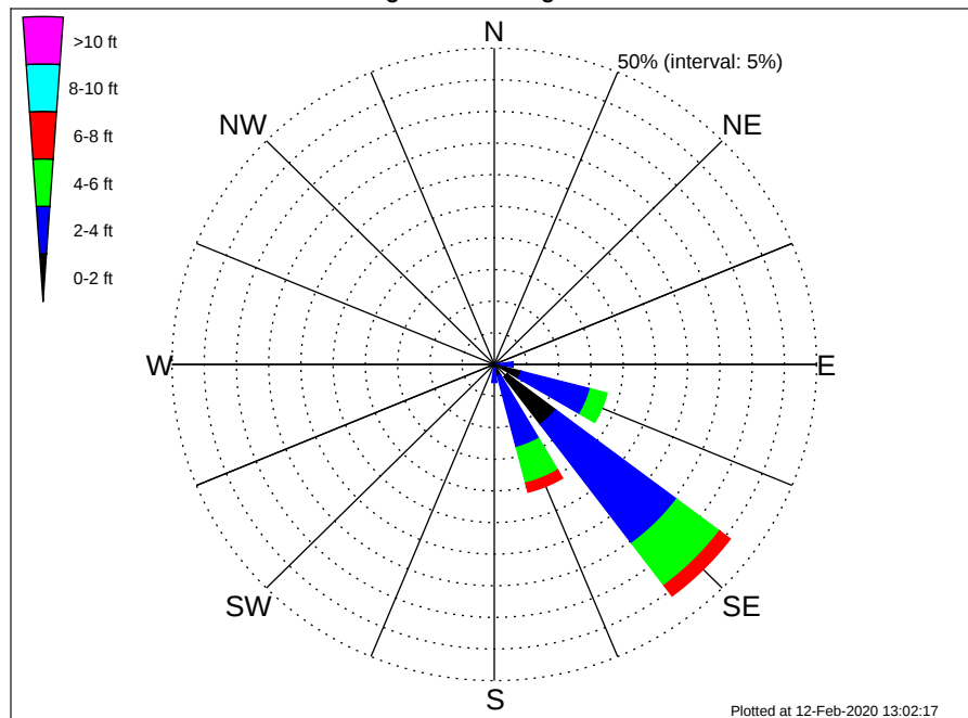
Flower Gardens NMS Climatological WaveHeight Rose for June: 1979 - 2015
