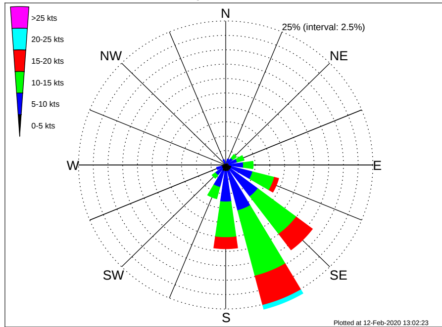
Flower Gardens NMS Climatological Wind Rose for June: 1979 - 2015
