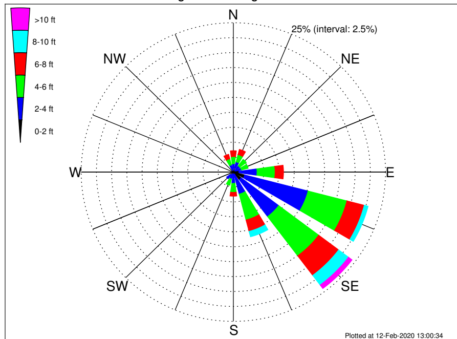
Flower Gardens NMS Climatological WaveHeight Rose for March: 1979 - 2015
