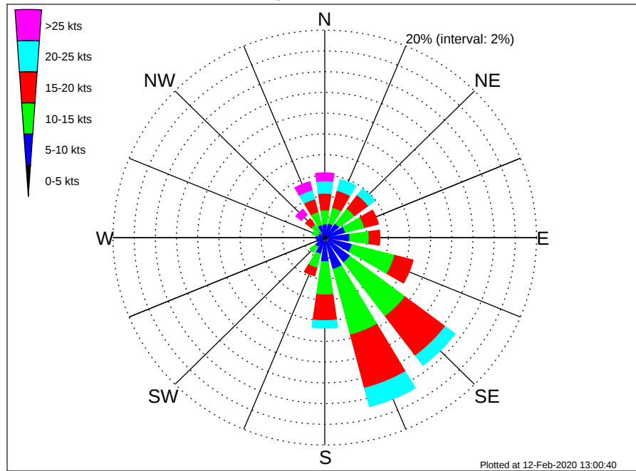
Flower Gardens NMS Climatological Wind Rose for March: 1979 - 2015
