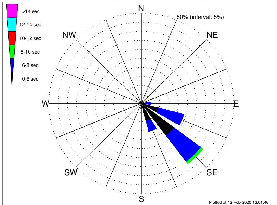
Flower Gardens NMS Climatological WavePeriod Rose for May: 1979 - 2015
