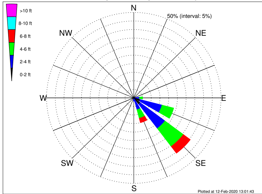
Flower Gardens NMS Climatological WaveHeight Rose for May: 1979 - 2015
