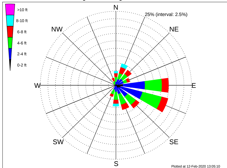
Flower Gardens NMS Climatological WaveHeight Rose for November: 1979 - 2015
