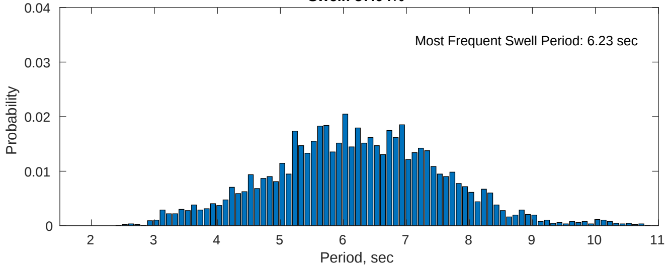
Swell: 57.04%
