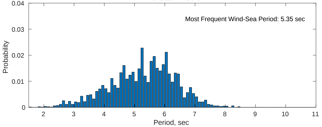
Wind-Sea: 42.96%
