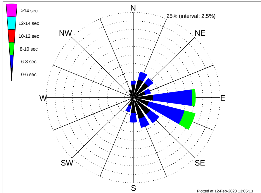
Flower Gardens NMS Climatological WavePeriod Rose for November: 1979 - 2015
