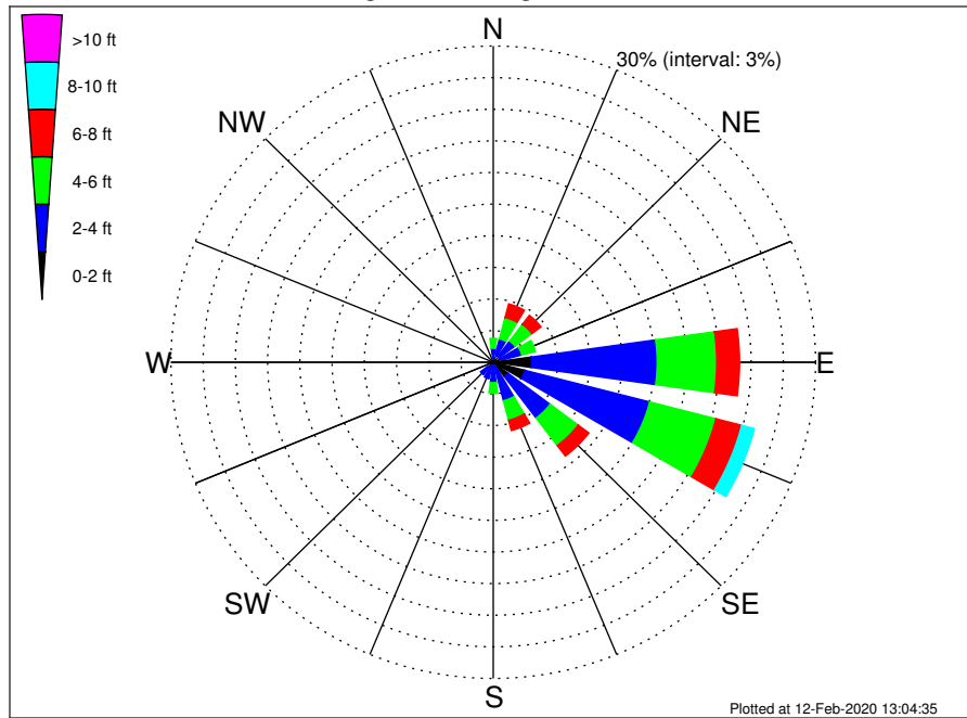
Flower Gardens NMS Climatological WaveHeight Rose for October: 1979 - 2015
