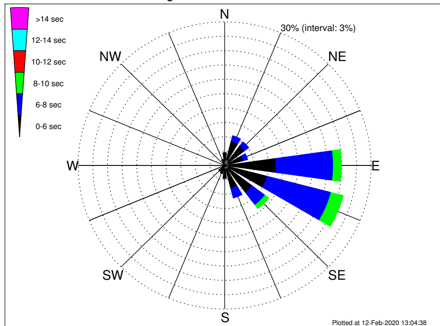
Flower Gardens NMS Climatological WavePeriod Rose for October: 1979 - 2015
