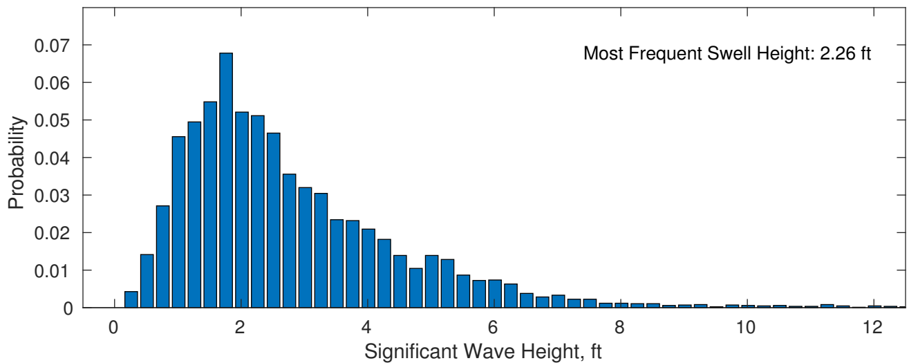
Swell: 70.96%
