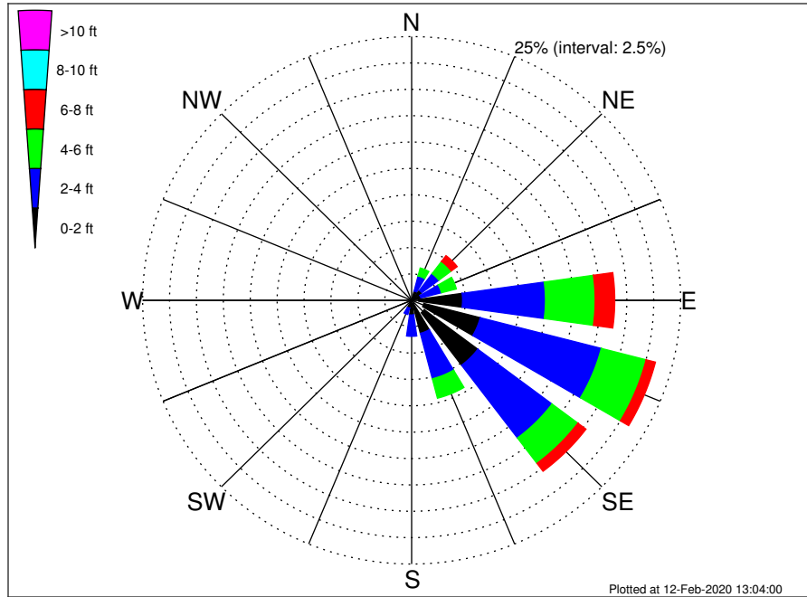
Flower Gardens NMS Climatological WaveHeight Rose for September: 1979 - 2015
