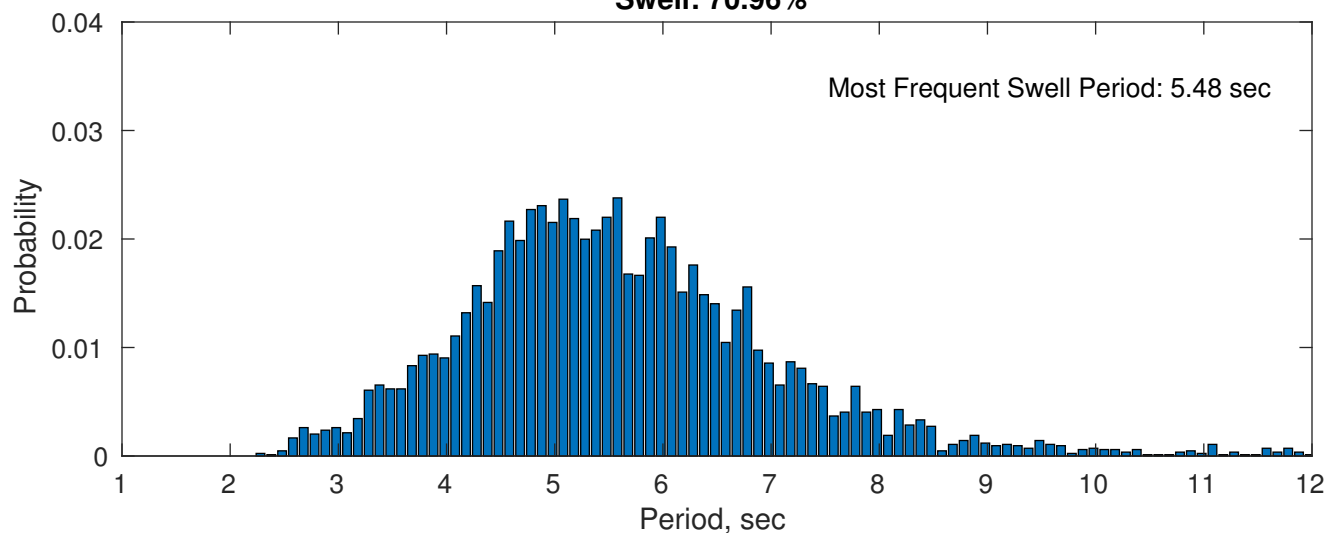
Swell: 70.96%
