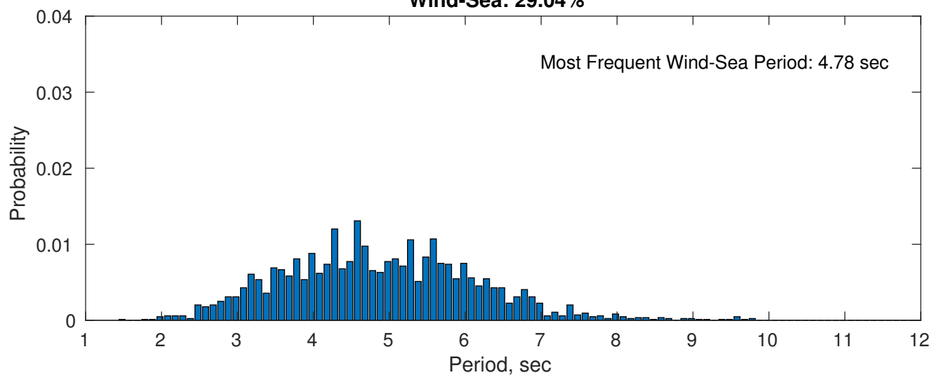
Wind-Sea: 29.04%
