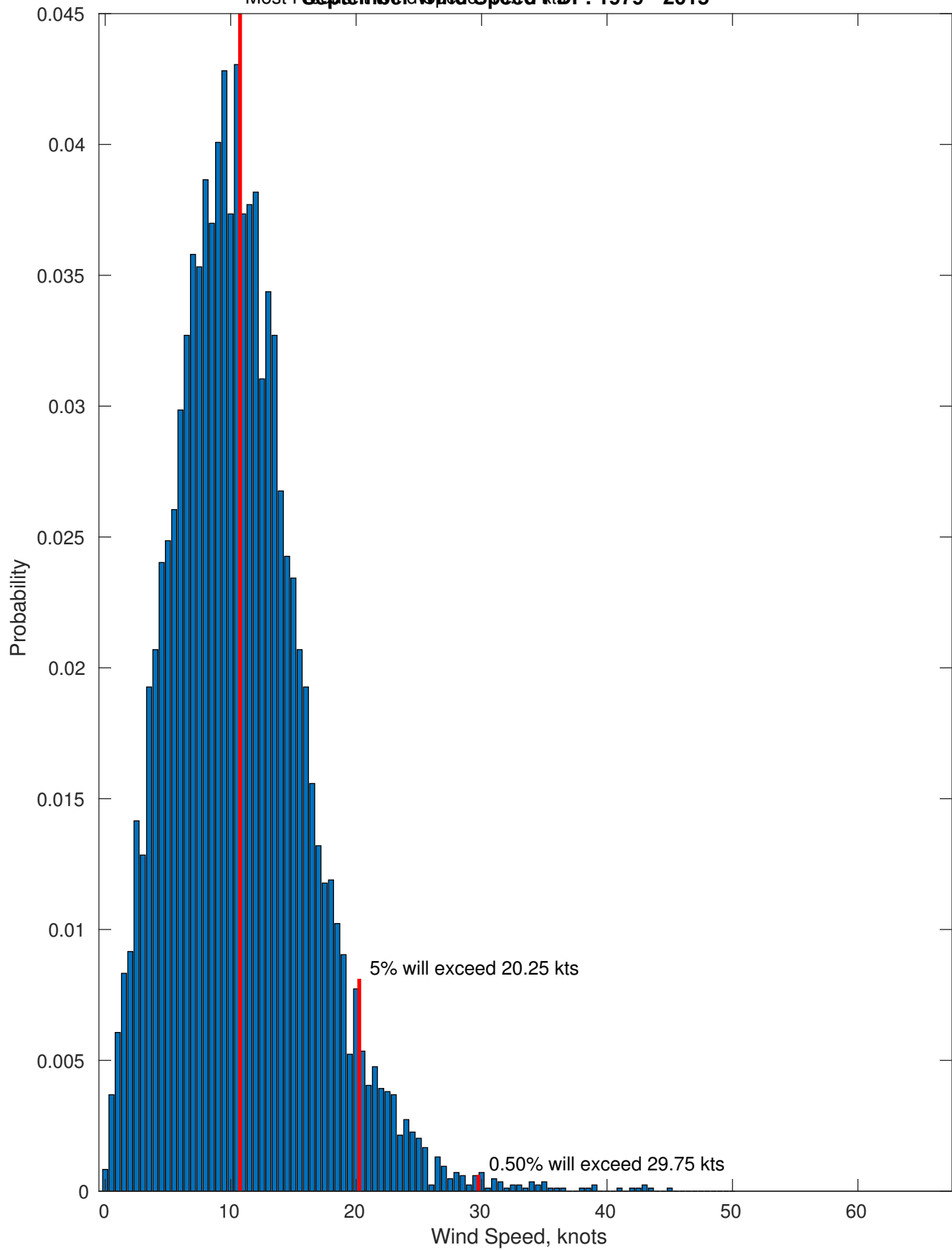
Most Frequent Wind Speed PDF: 1979 - 2015
