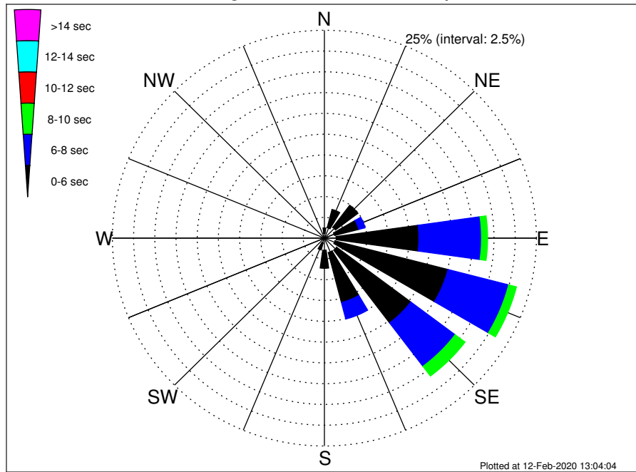
Flower Gardens NMS Climatological WavePeriod Rose for September: 1979 - 2015
