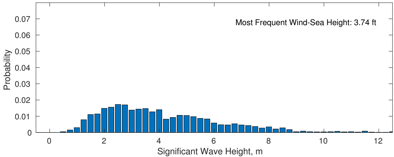
Wind-Sea: 29.04%
