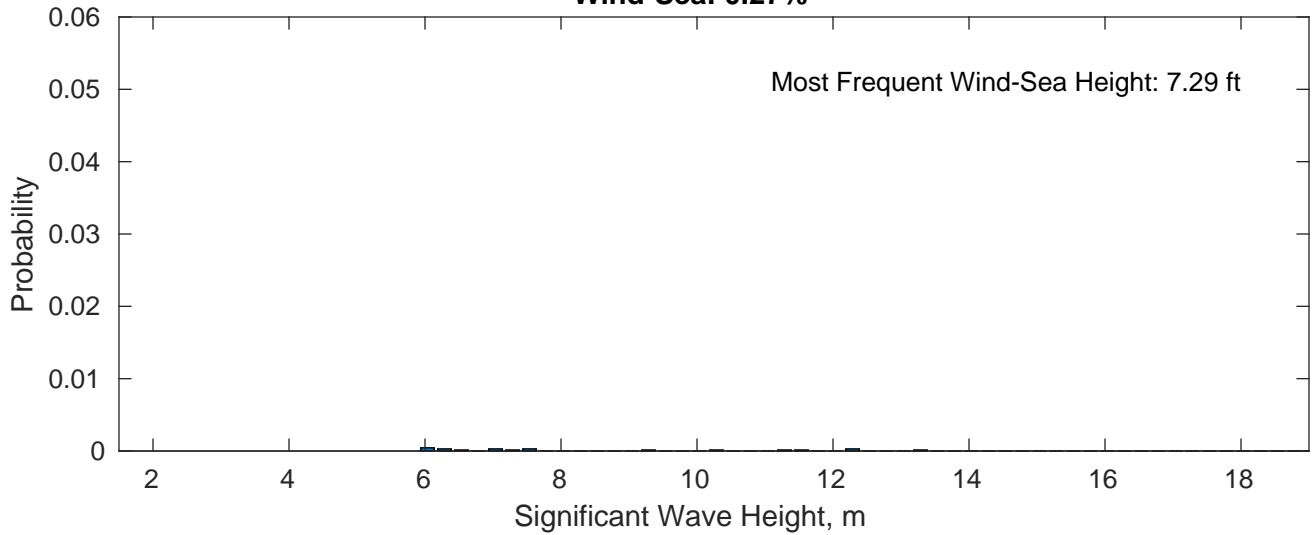
Wind-Sea: 0.27%
