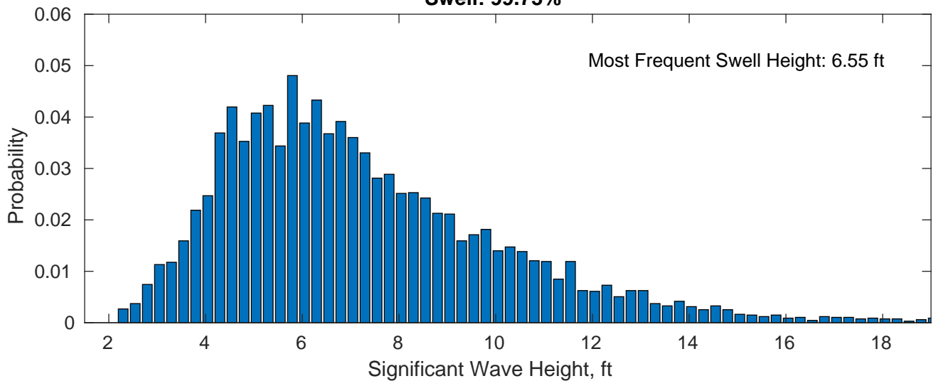
Swell: 99.73%
