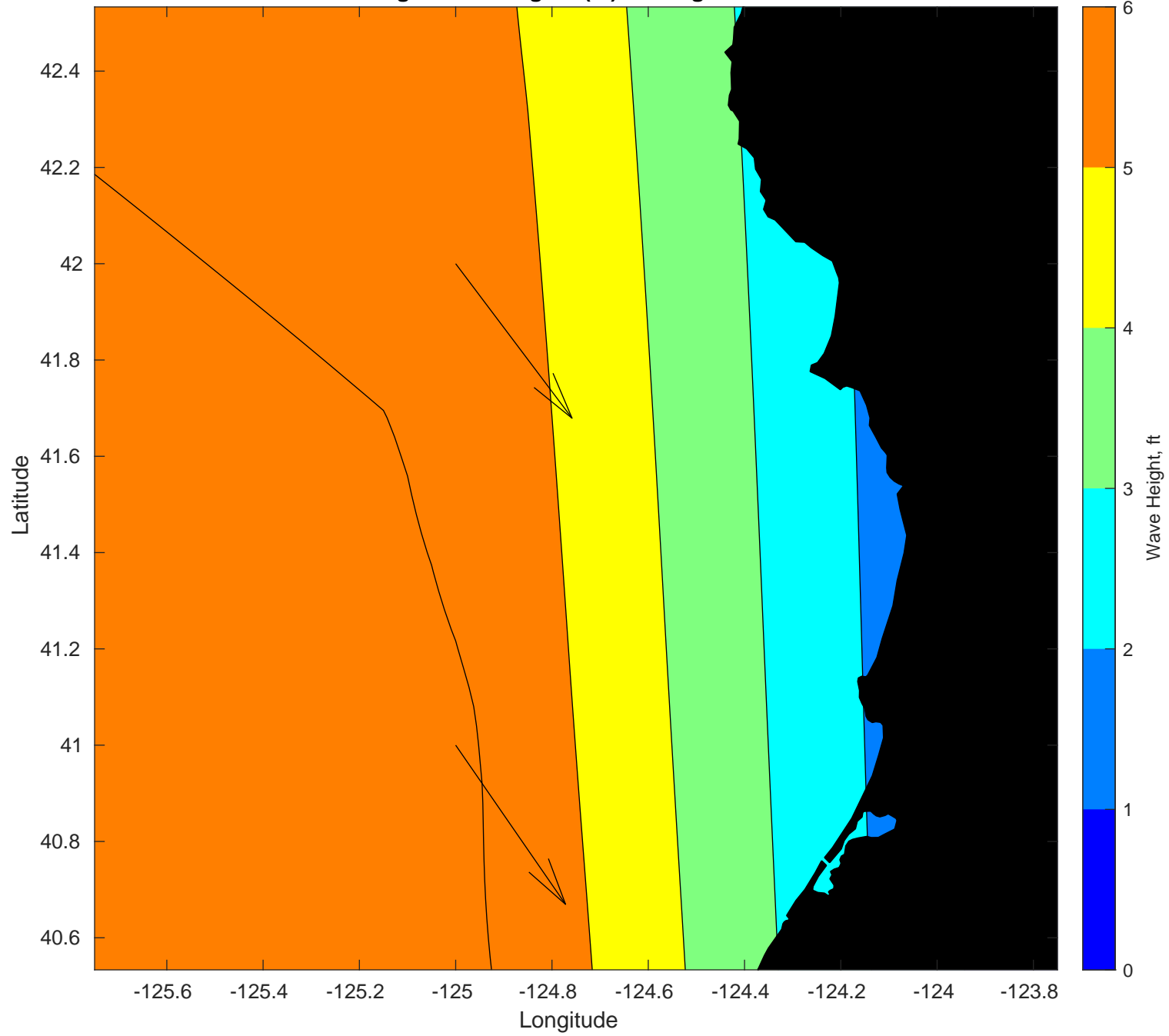
Average Wave Heights (m) for August
