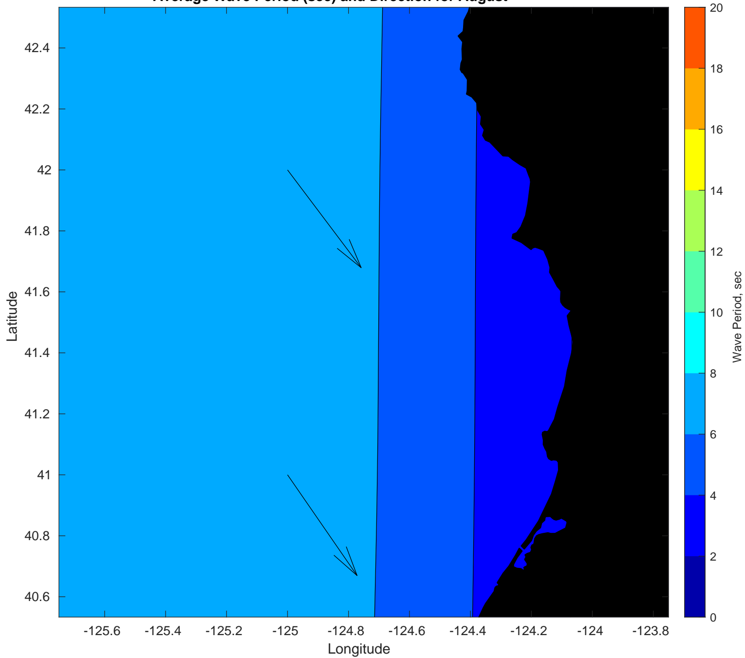
Average Wave Period (sec) and Direction for August
