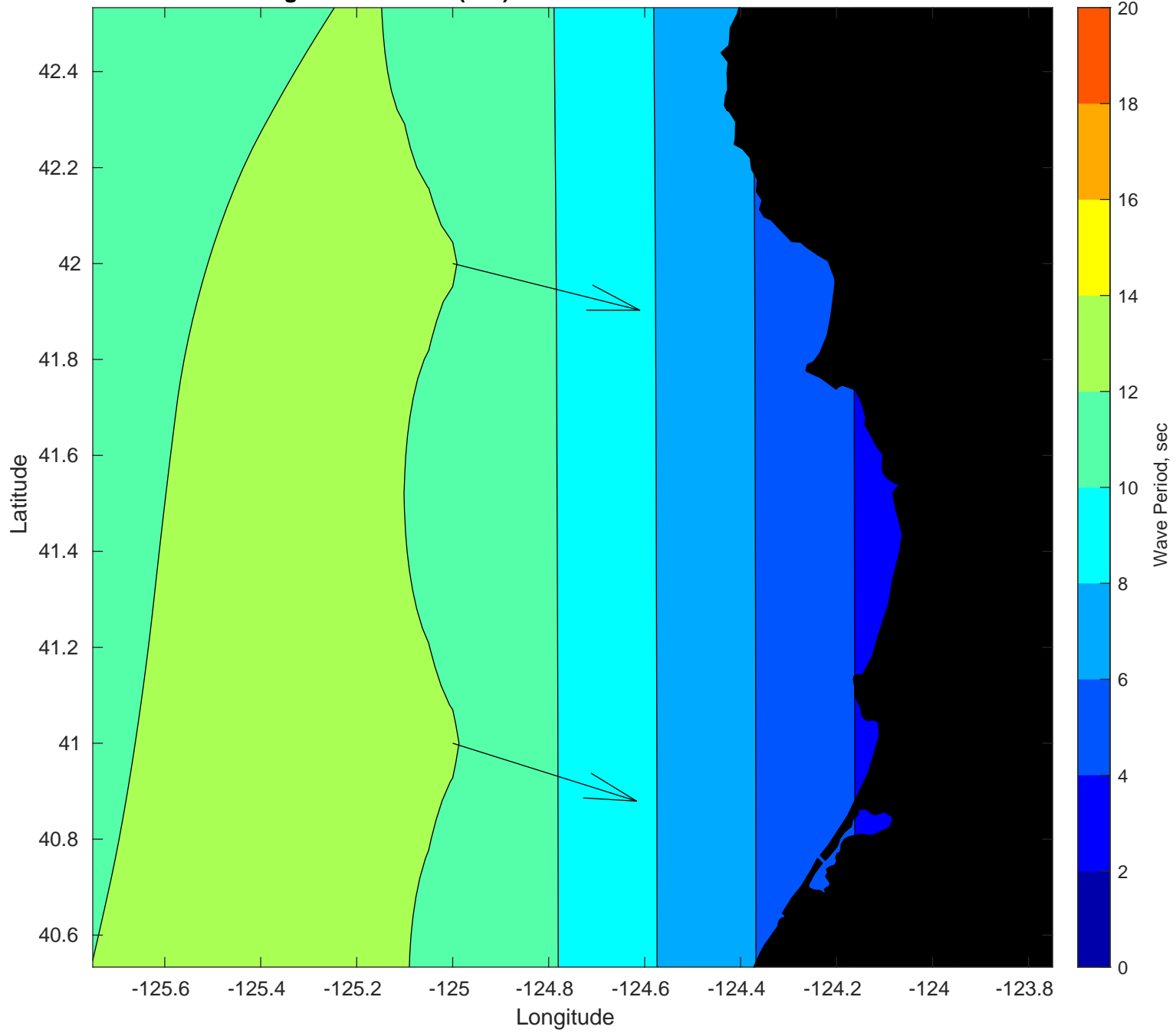
Average Wave Period (sec) and Direction for December
