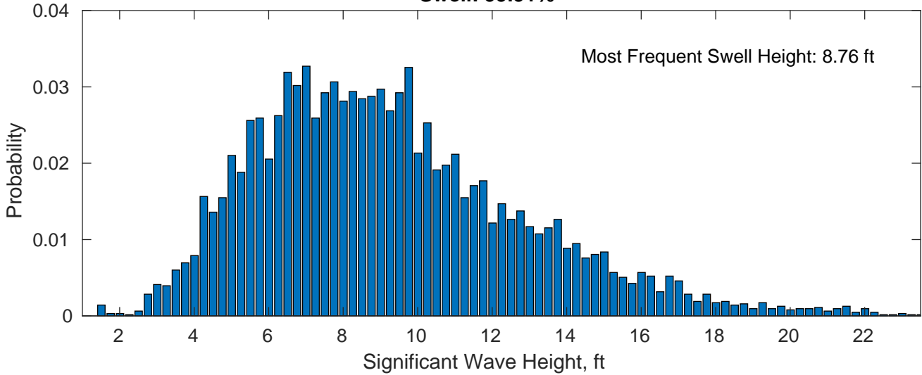
Swell: 99.91%
