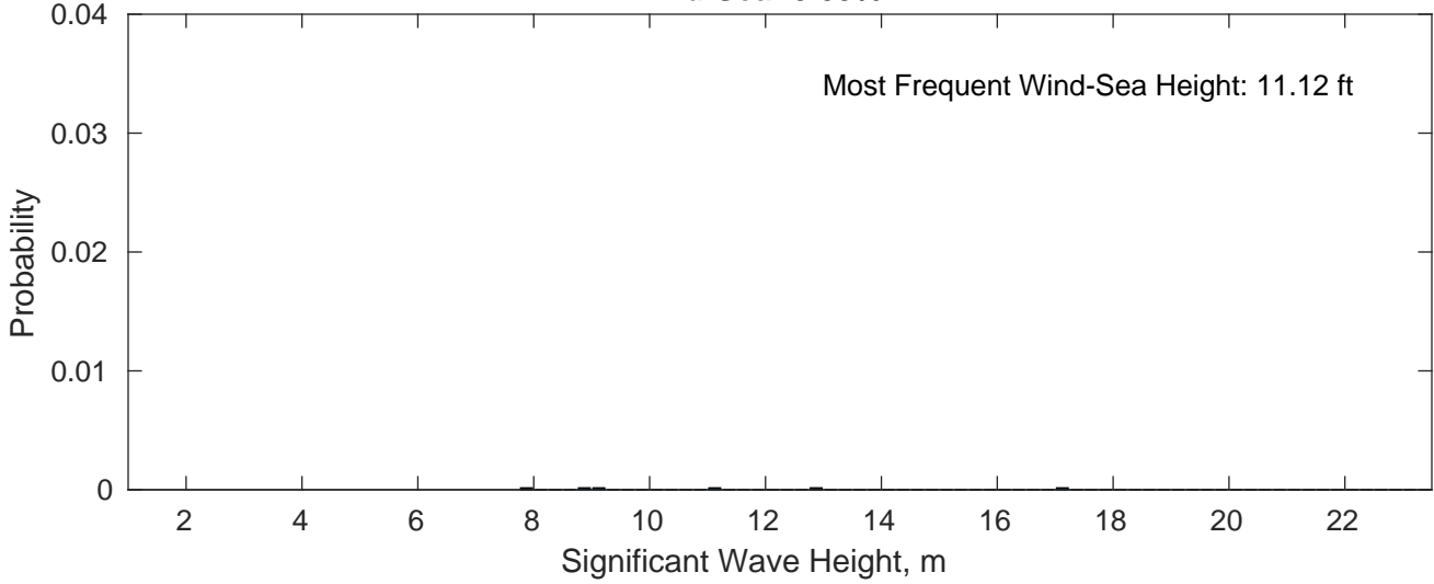
Wind-Sea: 0.09%
