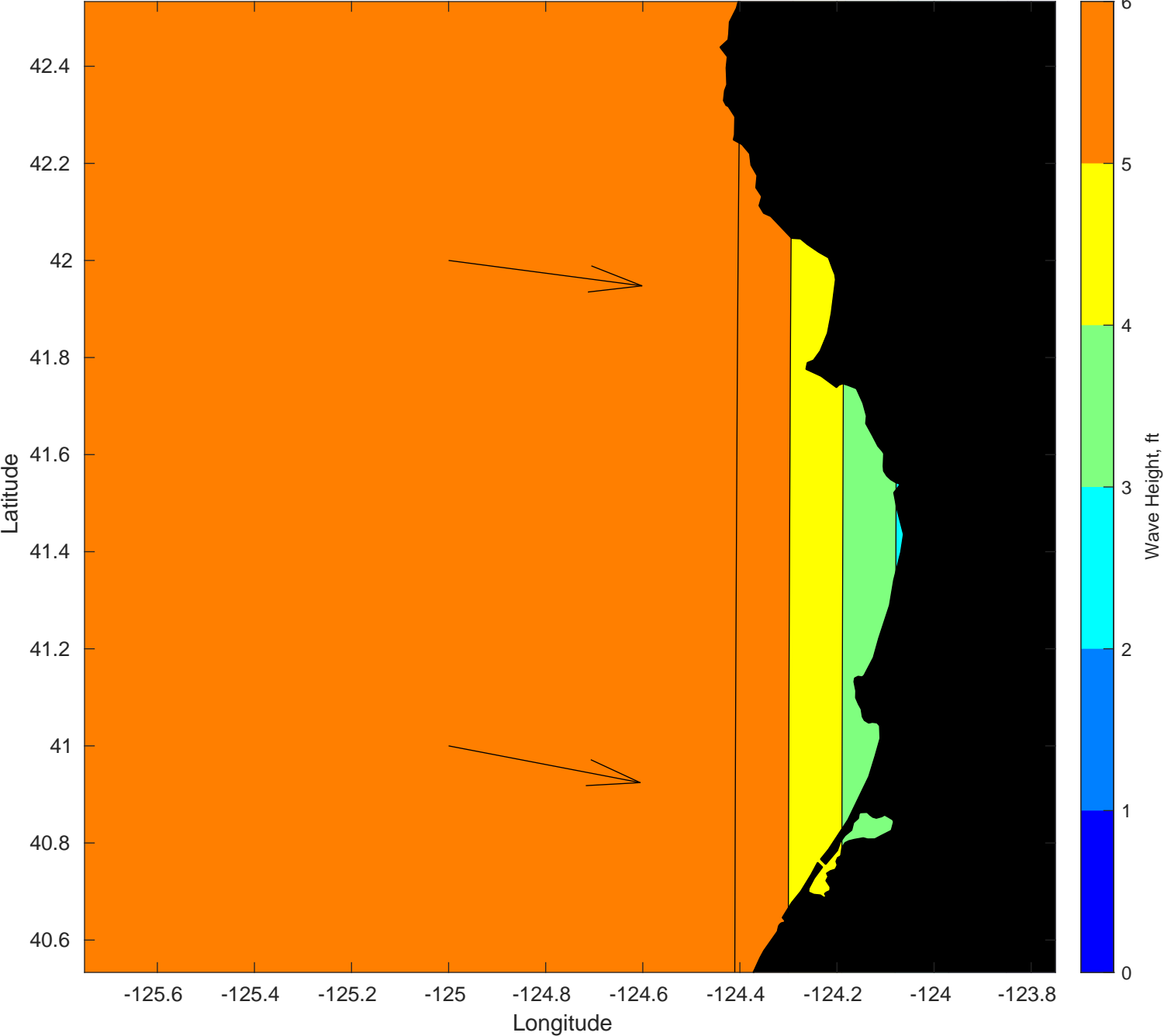
Average Wave Heights (m) for January
