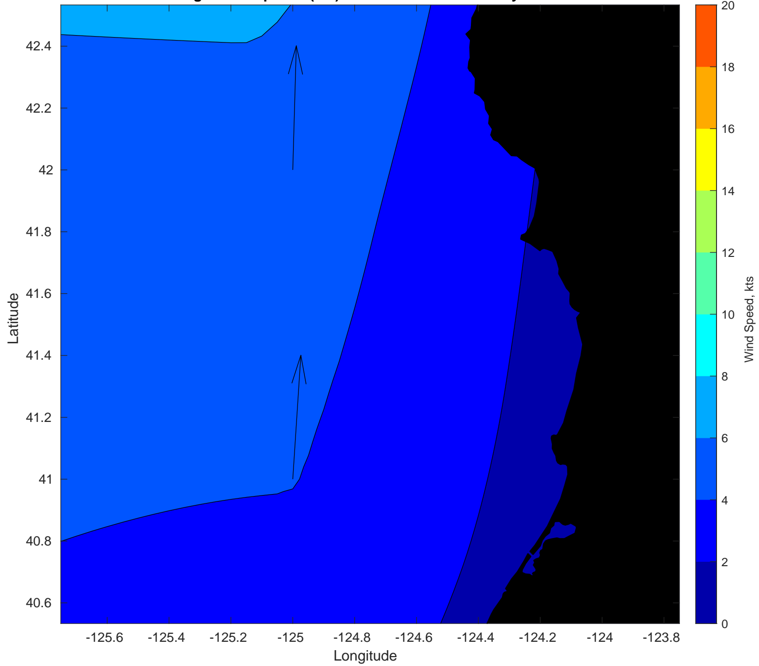
Average Wind Speeds (kts) and Direction for January
