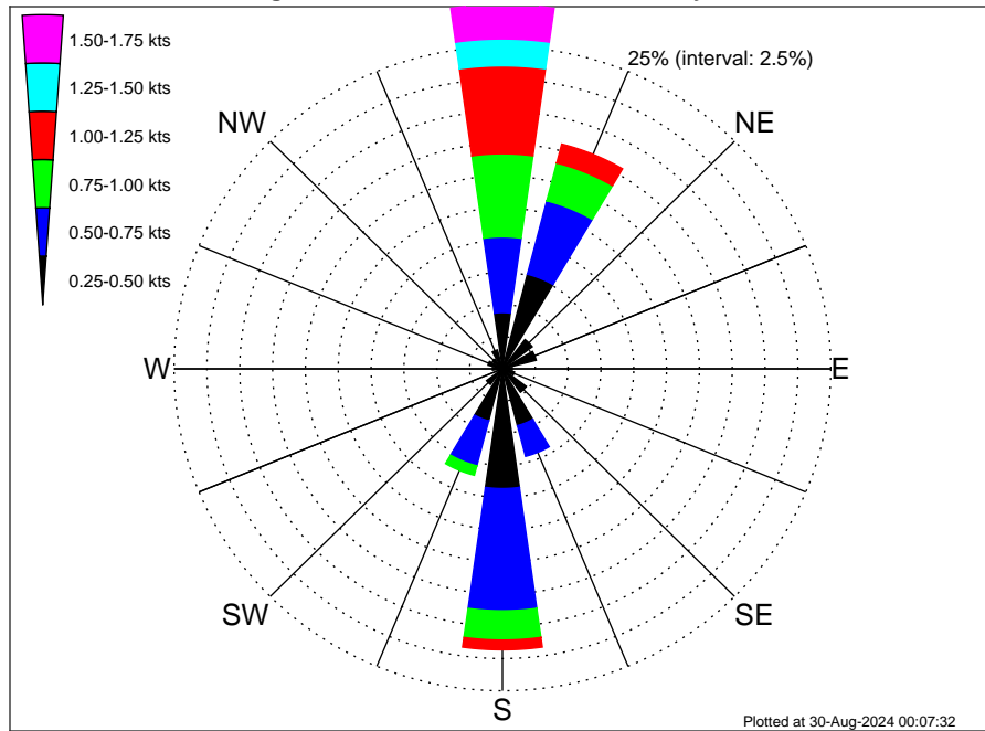
Klamath Slide Climatological Surface Current Rose for January: 1995 - 2012
