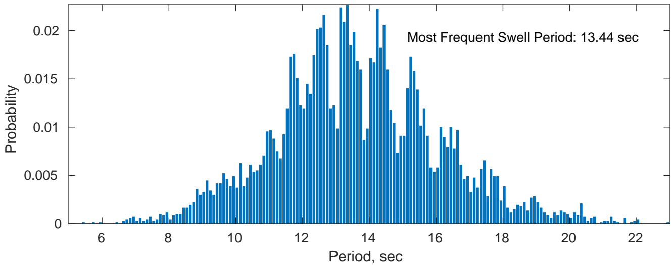
Swell: 99.70%
