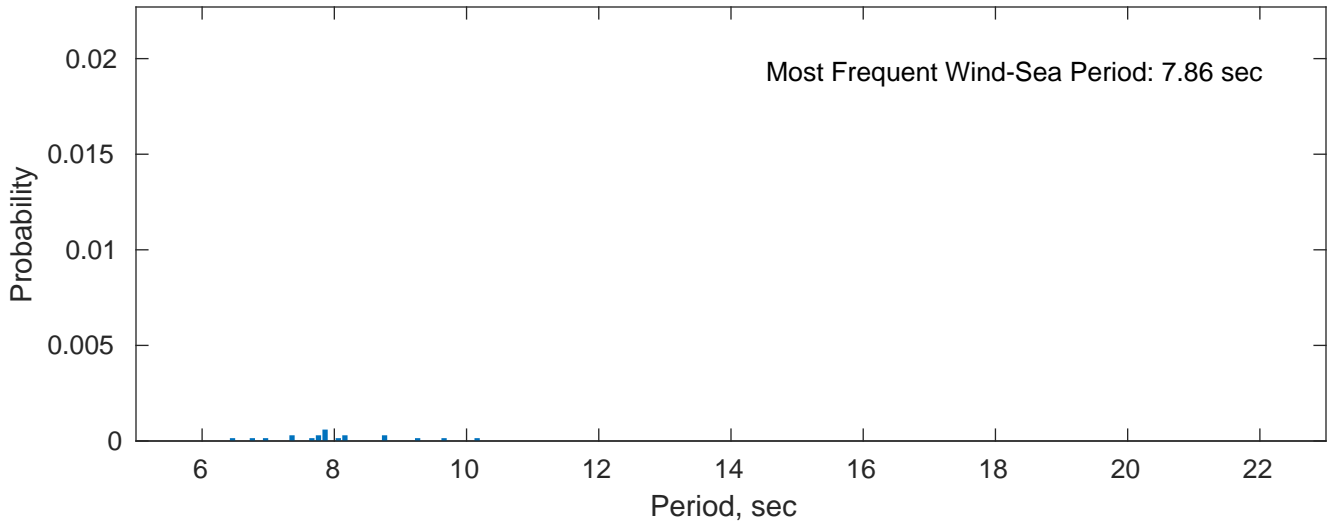
Wind-Sea: 0.30%
