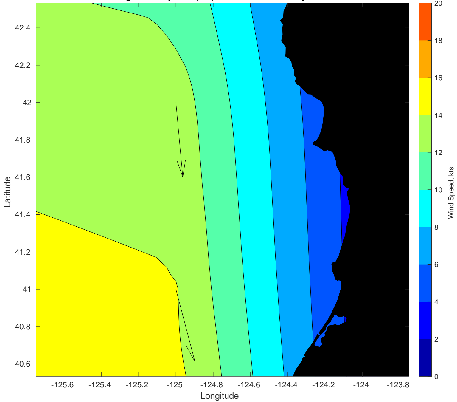
Average Wind Speeds (kts) and Direction for July
