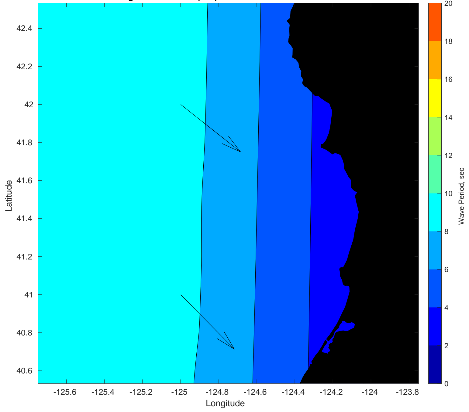
Average Wave Period (sec) and Direction for June
