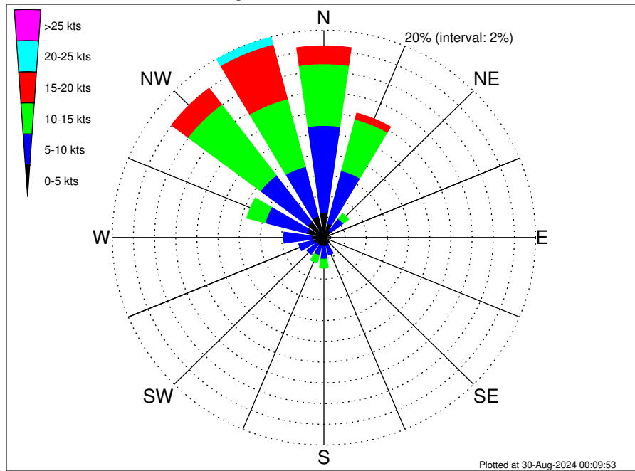
Klamath Slide Climatological Wind Rose for June: 1979 - 2015
