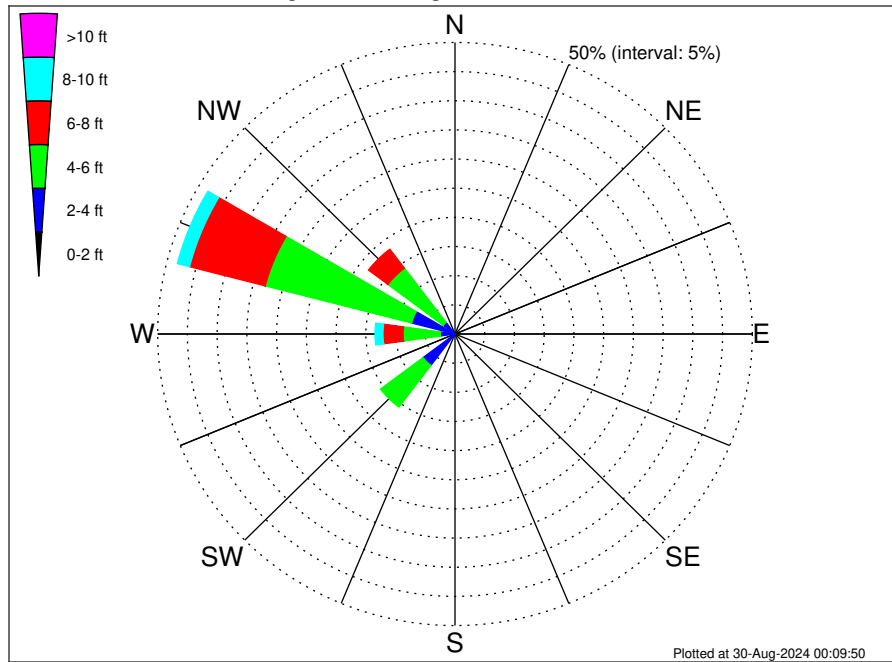
Klamath Slide Climatological WaveHeight Rose for June: 1979 - 2015
