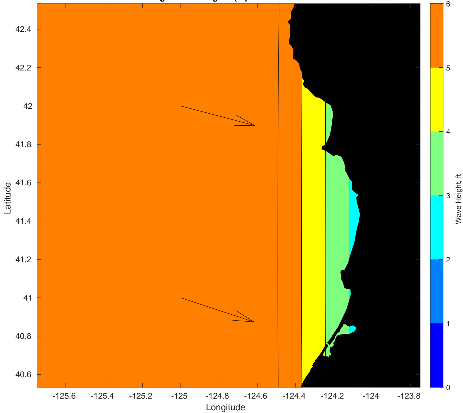
Average Wave Heights (m) for March
