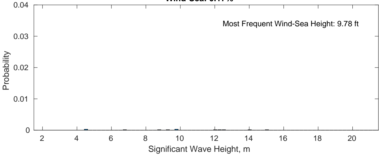
Wind-Sea: 0.17%
