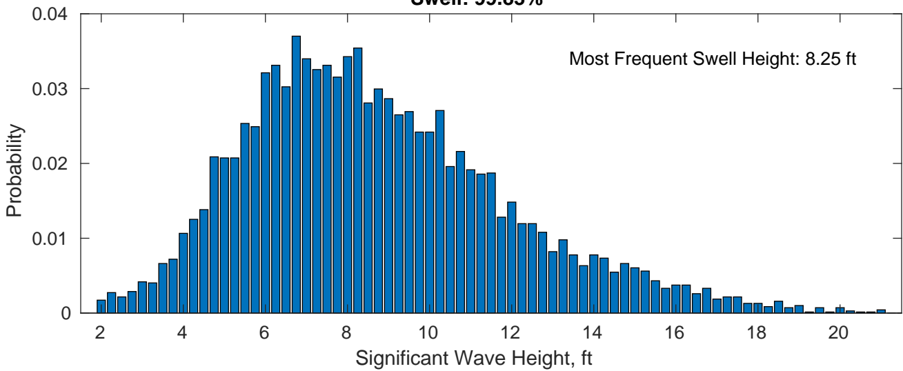
Swell: 99.83%
