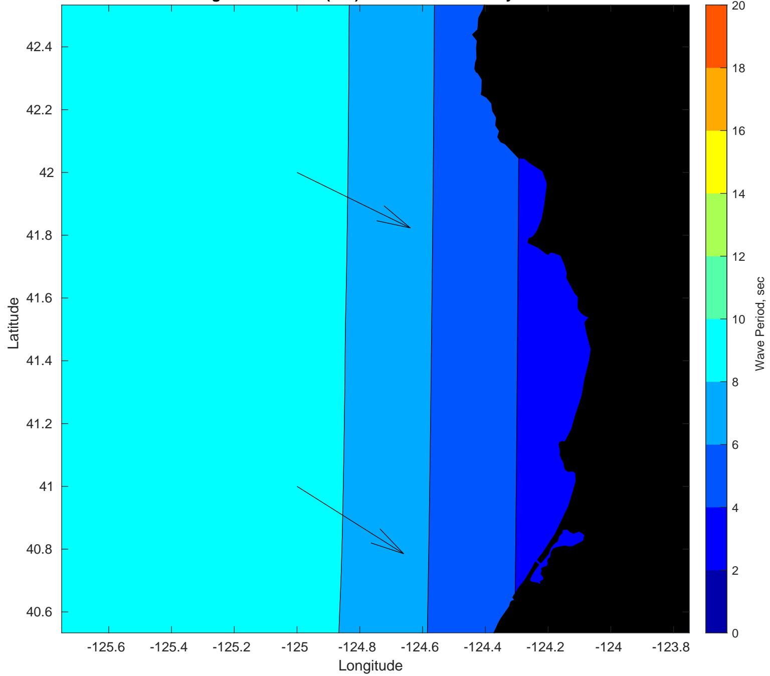
Average Wave Period (sec) and Direction for May
