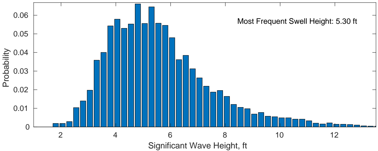
Swell: 99.44%
