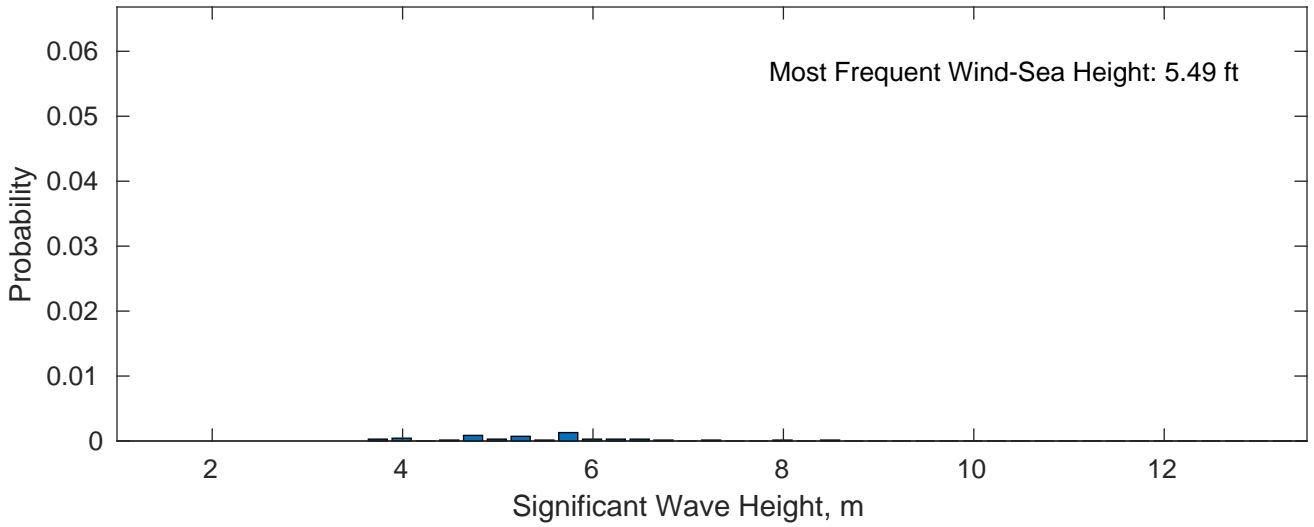
Wind-Sea: 0.56%
