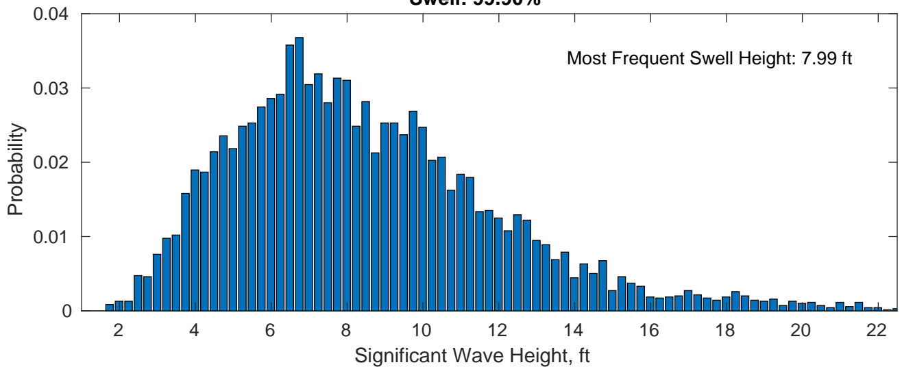
Swell: 99.90%
