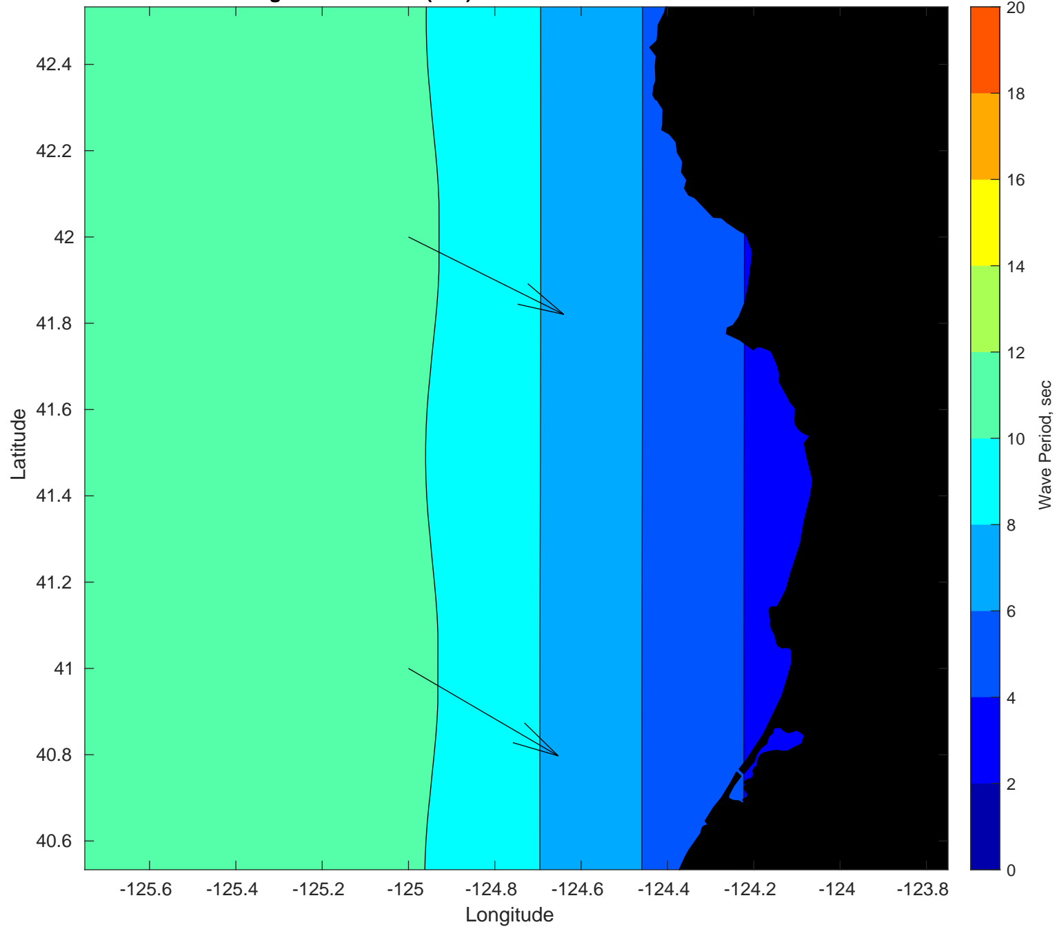
Average Wave Period (sec) and Direction for October
