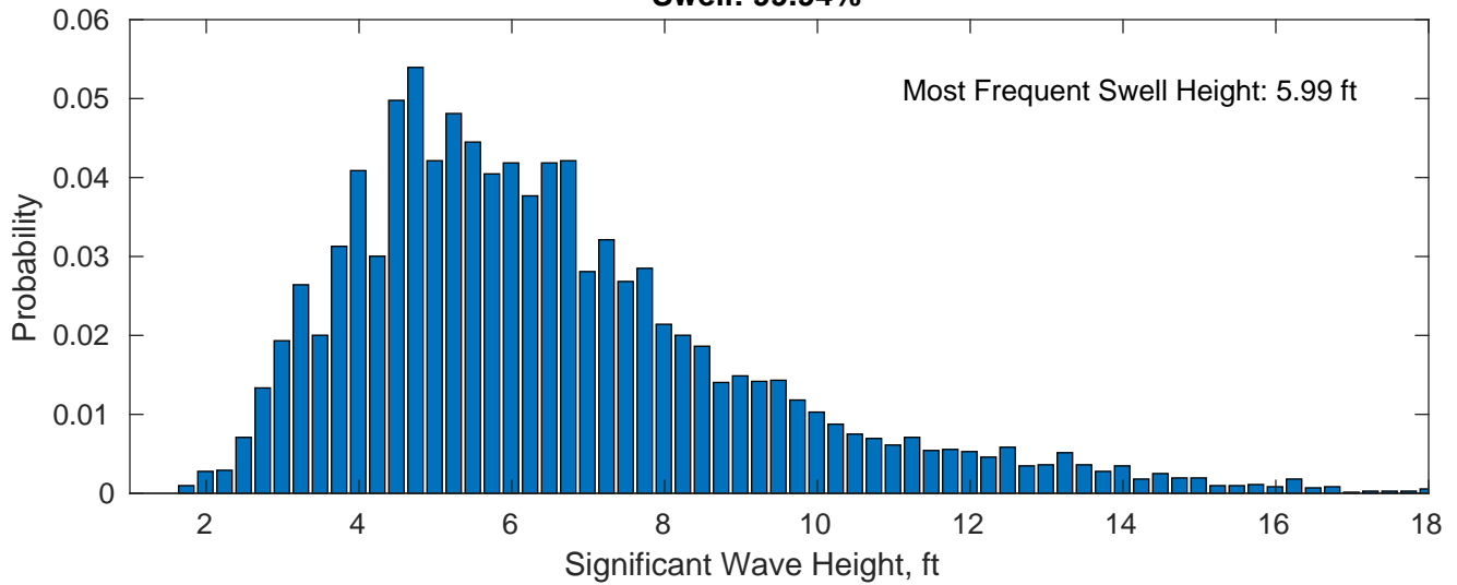
Swell: 99.94%
