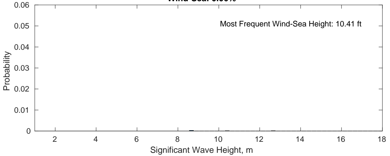
Wind-Sea: 0.06%
