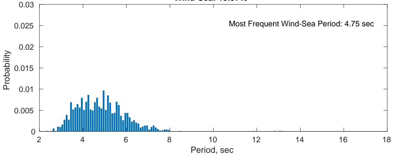
Wind-Sea: 19.97%
