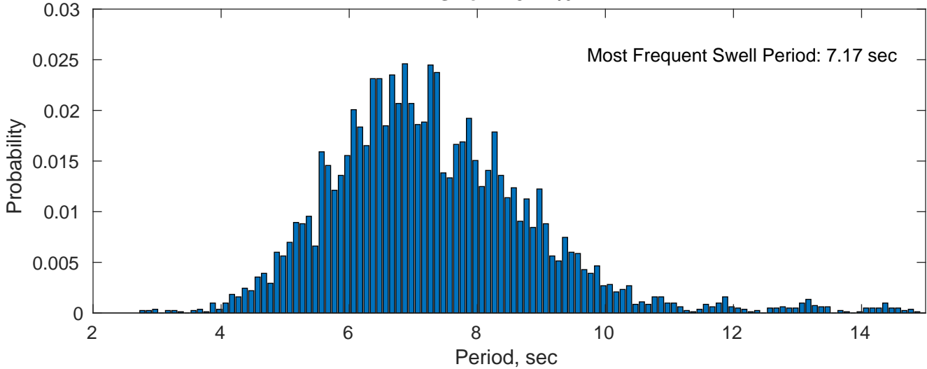
Swell: 75.41%
