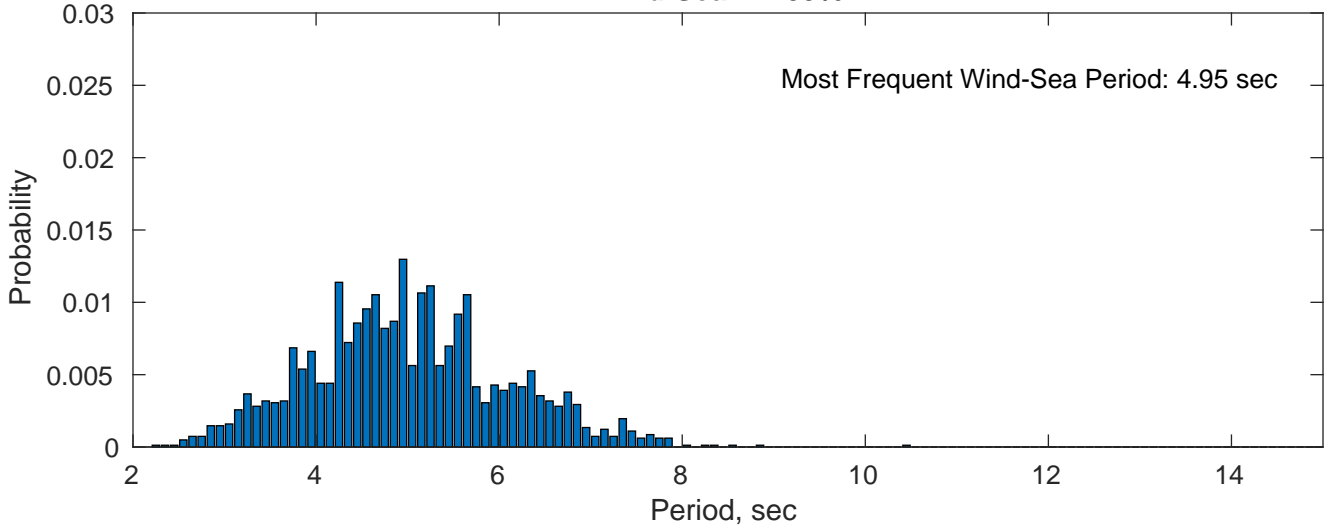
Wind-Sea: 24.59%
