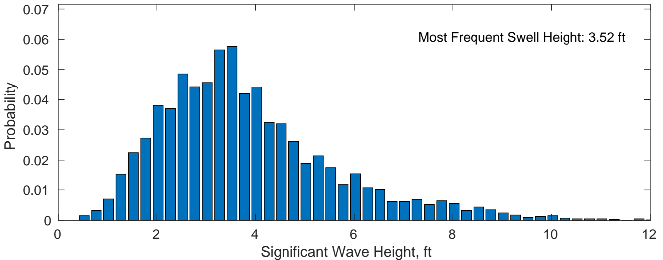
Swell: 74.53%
