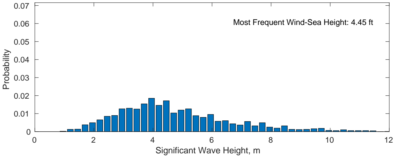
Wind-Sea: 25.47%
